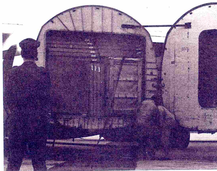
Pictured above, the arrival of the Argosy aircraft at Prague Airport, which was chartered from Air Bridge Carriers Ltd., of Castle Donnington, by Redifon Computers Ltd. The aircraft was loaded with R-range equipment for delivery to VZKG [four R830's]; Savings Bank, Plzen [one R300]; Supro [one R850] and Bastro [one R850].
